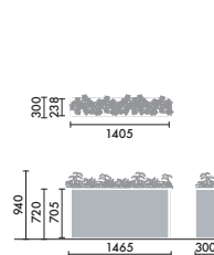
Planter box and artificial plants
