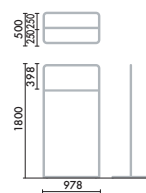
Coat hanger type
